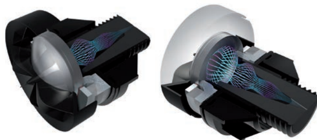
Figure 24 Front and rear view cross sections of tweeter showing rear loading
